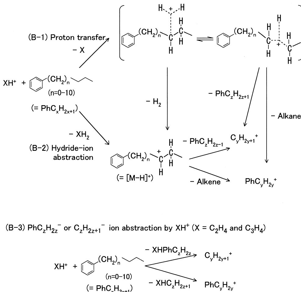
Scheme 2. Reaction scheme of the ion-molecule reactions of \text{XH}^+ ( \text{X} = \text{CH}_4 , \text{C}_2\text{H}_4 , and \text{C}_3\text{H}_4 ) with alkylbenzenes for attack of the reactant ion on the alkyl chain.
