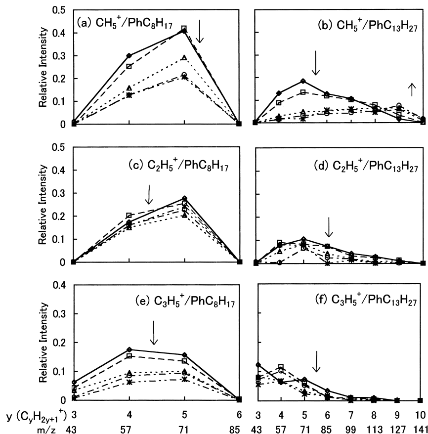
Fig. 1. Dependence of product-ion distributions of C_yH_{2y+1}^+ ( y = 3-10 ) ion on the reaction time in the ion-molecule reactions of CH_5^+ , C_2H_5^+ , and C_3H_5^+ with PhC_8H_{17} and PhC_{13}H_{27} . Reaction time \diamond : 0.5, \square : 2, \triangle : 10, \circ : 20, and \times : 40 ms. Relative intensities were branching ratios of each ion for total product ions. Arrows indicate an increase or a decrease in product-ion distribution with an increasing the reaction time. The line connecting the points in the graphs is the C_yH_{2y+1}^+ formed from the same reaction time.
