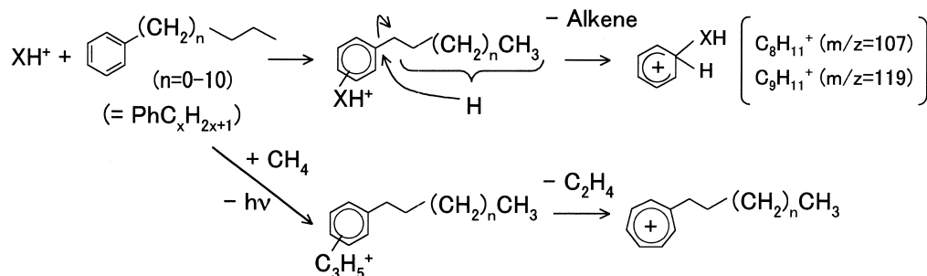
Scheme 1. Reaction scheme of the ion-molecule reactions of XH^+ ( X = CH_4, C_2H_4 , and C_3H_4 ) with alkylbenzenes for attack of the reactant ion on the benzene ring.
