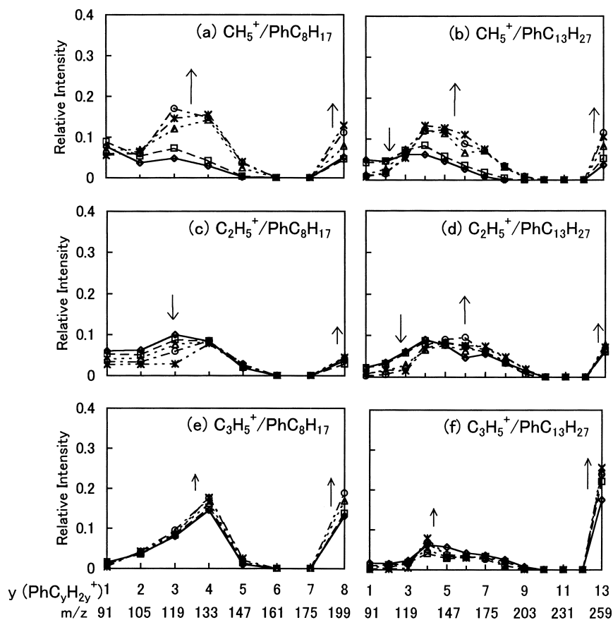
Fig. 2. Dependence of product-ion distributions of \text{PhC}_y\text{H}_{2y+1}^+ ( y = 1-13 ) ion on the reaction time in the ion-molecule reactions of \text{CH}_5^+ , \text{C}_2\text{H}_5^+ , and \text{C}_3\text{H}_5^+ with \text{PhC}_8\text{H}_{17} and \text{PhC}_{13}\text{H}_{27} . Reaction time \diamond : 0.5, \square : 2, \triangle : 10, \circ : 20, and \times : 40 ms. Relative intensities were branching ratios of each ion for total product ions. Arrows indicate an increase or a decrease in product-ion distribution with an increasing the reaction time. The line connecting the points in the graphs is the \text{PhC}_y\text{H}_{2y+1}^+ formed from the same reaction time.
