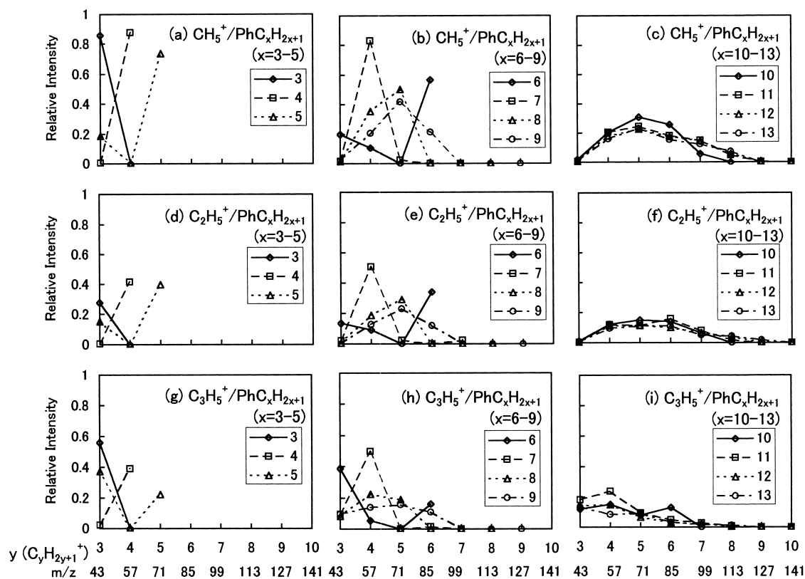
Fig. 3. Initial product-ion distributions of C_yH_{2y+1}^+ ( y = 3-10 ) ion in the ion-molecule reactions of CH_5^+ , C_2H_5^+ , and C_3H_5^+ with C_9 - C_{19} alkylbenzenes. (a), (d), (g) \diamond : PhC_3H_7 , \square : PhC_4H_9 , and \triangle : PhC_5H_{11} , (b), (e), (h) \diamond : PhC_6H_{13} , \square : PhC_7H_{15} , \triangle : PhC_8H_{17} , and \circ : PhC_9H_{19} , (c), (f), (i) \diamond : PhC_{10}H_{21} , \square : PhC_{11}H_{23} , \triangle : PhC_{12}H_{25} , and \circ : PhC_{13}H_{27} . The largest C_yH_{2y+1}^+ ions correspond to the C_xH_{2x+1}^+ ions. The line connecting the points in the graphs is the alkyl C_yH_{2y+1}^+ ( y = 3-x ) ion formed from the same alkylbenzene.
