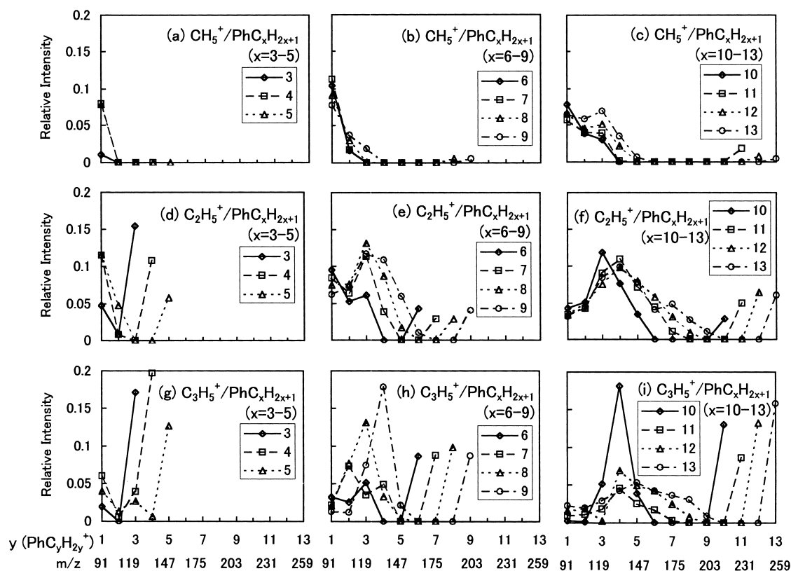
Fig. 4. Initial product-ion distributions of \text{PhC}_y\text{H}_{2y}^+ ( y = 1-13 ) ion in the ion-molecule reactions of \text{CH}_5^+ , \text{C}_2\text{H}_5^+ , and \text{C}_3\text{H}_5^+ with \text{C}_9 – \text{C}_{19} alkylbenzenes. (a), (d), (g) \diamond : \text{PhC}_3\text{H}_7 , \square : \text{PhC}_4\text{H}_9 , and \triangle : \text{PhC}_5\text{H}_{11} , (b), (e), (h) \diamond : \text{PhC}_6\text{H}_{13} , \square : \text{PhC}_7\text{H}_{15} , \triangle : \text{PhC}_8\text{H}_{17} , and \circ : \text{PhC}_9\text{H}_{19} , (c), (f), (i) \diamond : \text{PhC}_{10}\text{H}_{21} , \square : \text{PhC}_{11}\text{H}_{23} , \triangle : \text{PhC}_{12}\text{H}_{25} , and \circ : \text{PhC}_{13}\text{H}_{27} . The largest \text{PhC}_y\text{H}_{2y}^+ ions correspond to the \text{PhC}_x\text{H}_{2x}^+ ions. The line connecting the points in the graphs is the \text{PhC}_y\text{H}_{2y}^+ ( y = 1-13 ) ion formed from same alkylbenzene.
