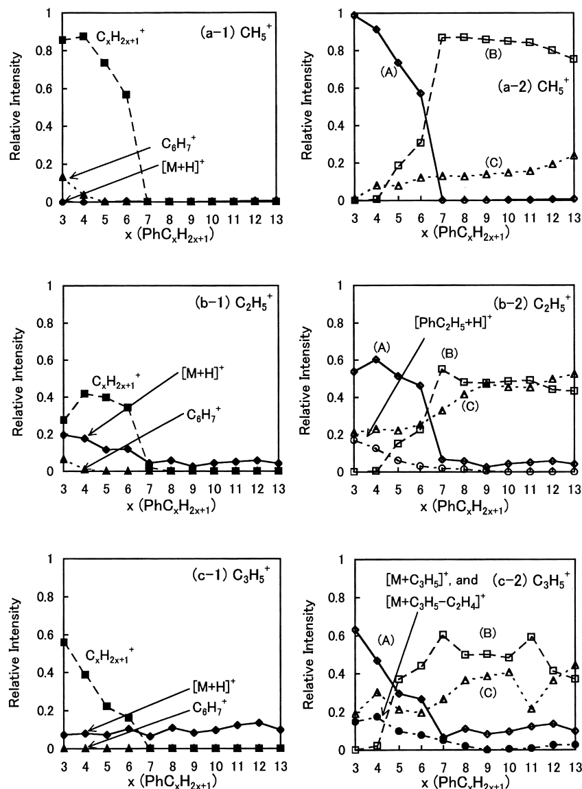
Fig. 6. Dependence of the branching ratios of product ions on the alkyl chain x in \text{PhC}_x\text{H}_{2x+1} . (a) \text{CH}_5^+ , (b) \text{C}_2\text{H}_5^+ , and (c) \text{C}_3\text{H}_5^+ .
