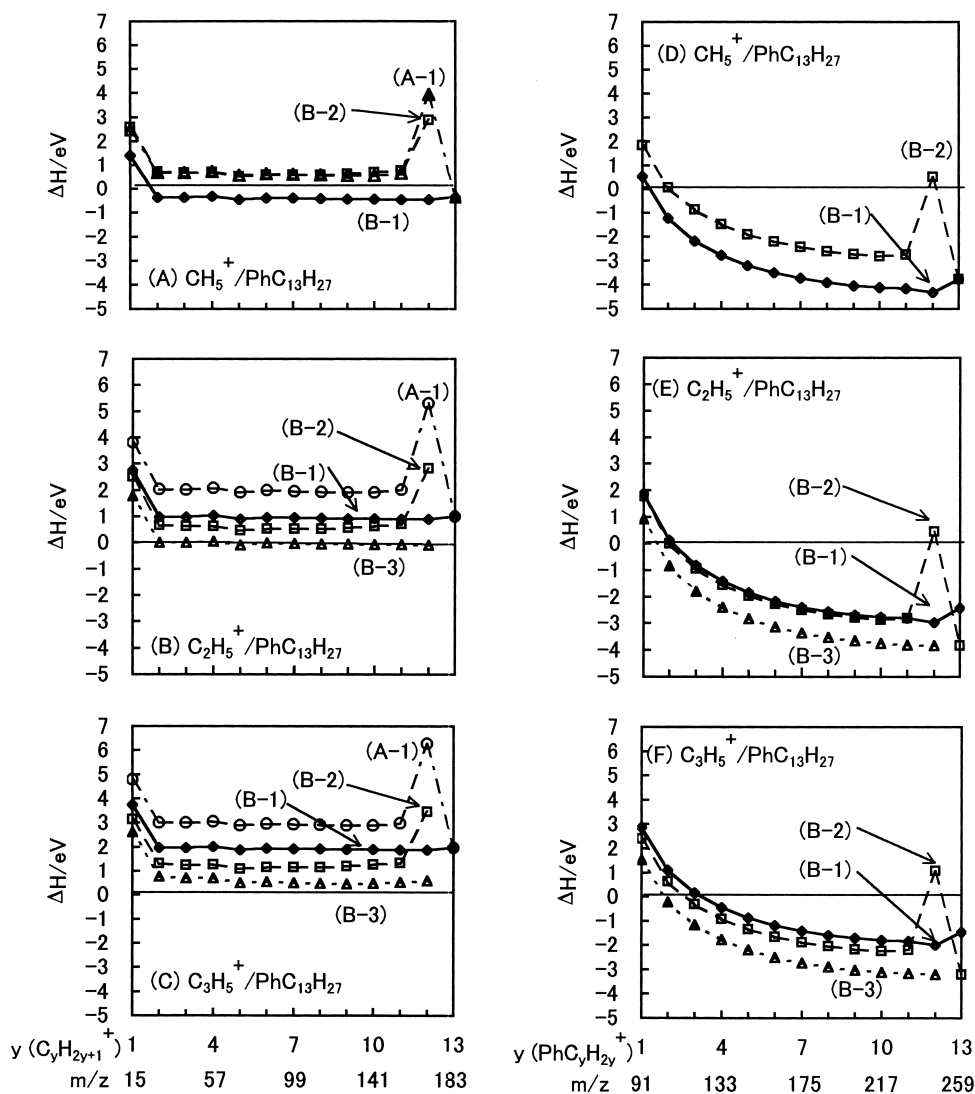
Fig. 5. Energy relations in the ion-molecule reactions of \text{CH}_5^+ , \text{C}_2\text{H}_5^+ , and \text{C}_3\text{H}_5^+ with \text{PhC}_{13}\text{H}_{27} leading to 1\text{-C}_y\text{H}_{2y+1}^+ and \text{PhC}_y\text{H}_{2y}^+ . \diamond : (1a) Proton transfer, \square : (2a) hydride-ion abstraction, \triangle : (3a) \text{PhC}_x\text{H}_{2x-} ion abstraction. The largest \text{C}_y\text{H}_{2y+1}^+ ions correspond to the \text{C}_x\text{H}_{2x+1}^+ ions. \diamond : (1b) Proton transfer, \square : (2b) hydride-ion abstraction, \triangle : (3b) \text{C}_x\text{H}_{2x+1}^- ion abstraction. The largest \text{PhC}_y\text{H}_{2y}^+ ions correspond to the \text{PhC}_x\text{H}_{2x}^+ ions. The line connecting the points in the graphs is the \text{C}_y\text{H}_{2y+1}^+ and \text{PhC}_y\text{H}_{2y}^+ formed from the same reaction pathway. \Delta H^\circ values are shown in eV units ( 1 \text{ eV} = 96.485 \text{ kJ mol}^{-1} ).
